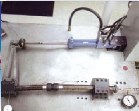
Figure 2: Fatigue testing
